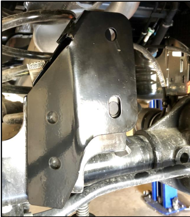
Driver Side Holes to Be Drilled
