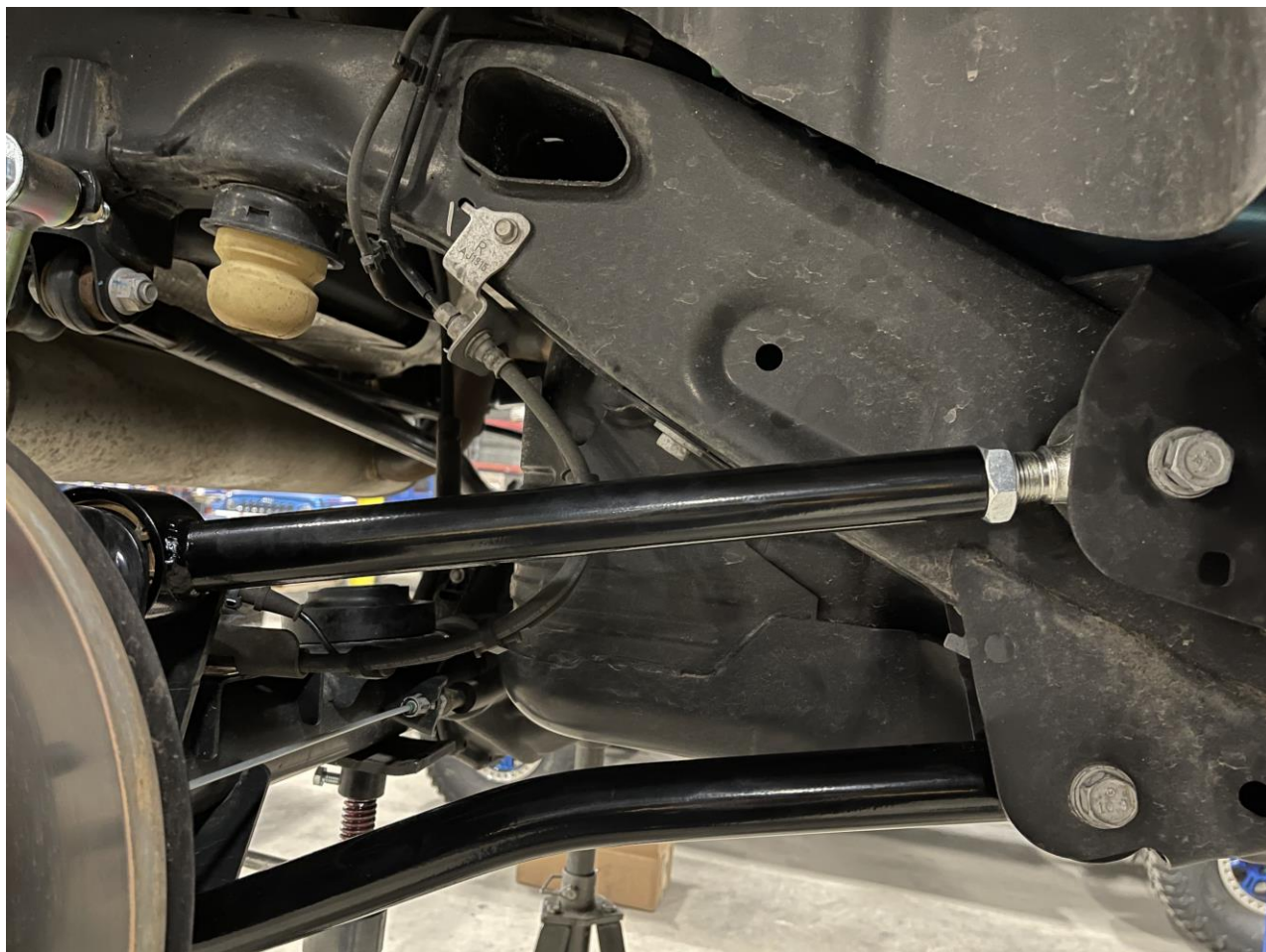
Rear Uppers and Rear Loweres Installed in the Vehicle
